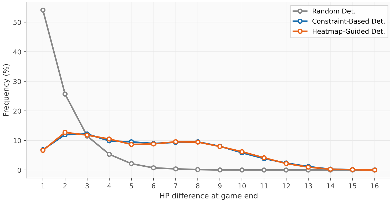
Game outcome margin distribution
