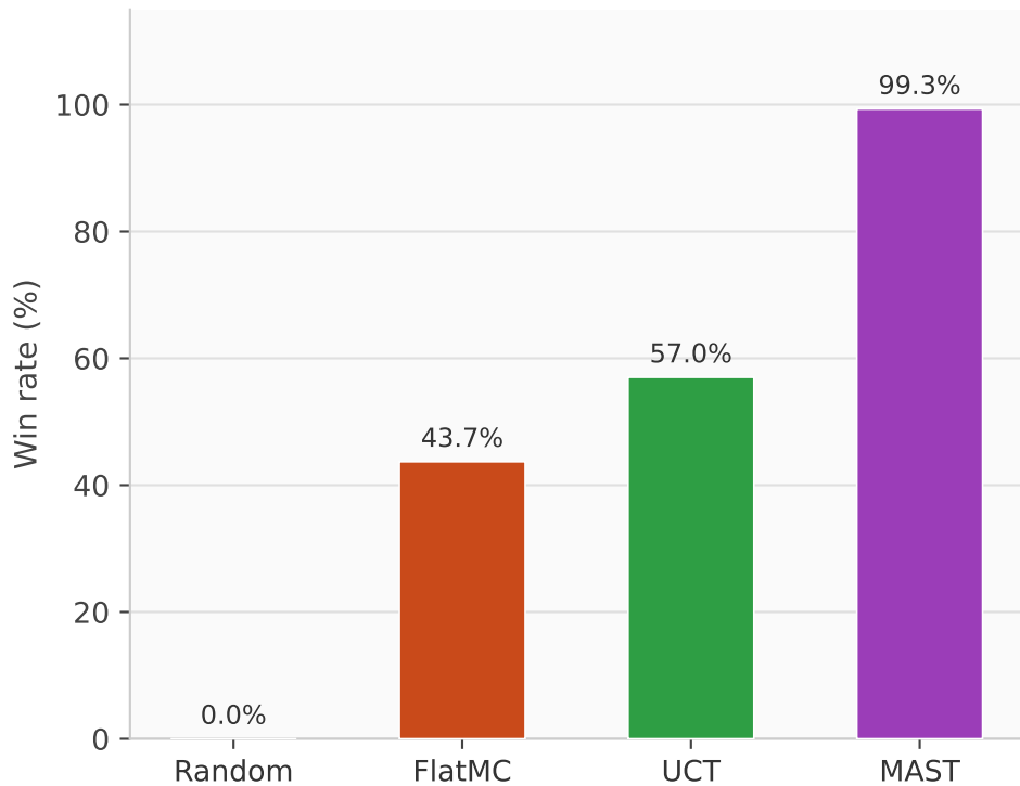
Win rates — Tournament 1 (native agents, no determinization)
