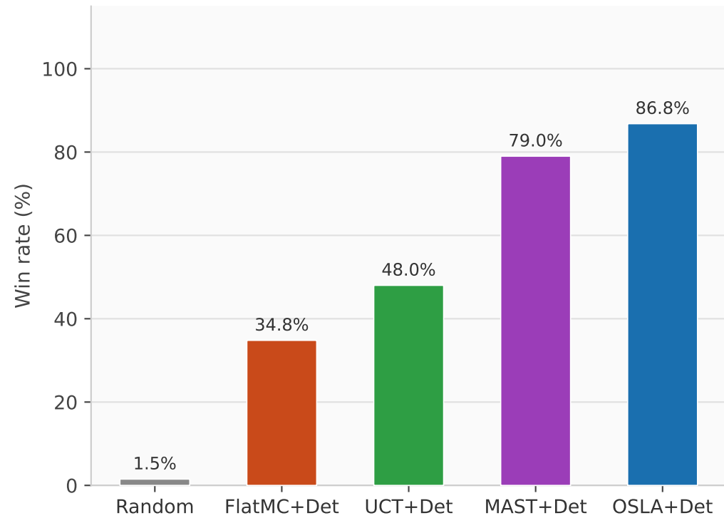
Win rates — Tournament 2 (determinized agents)
