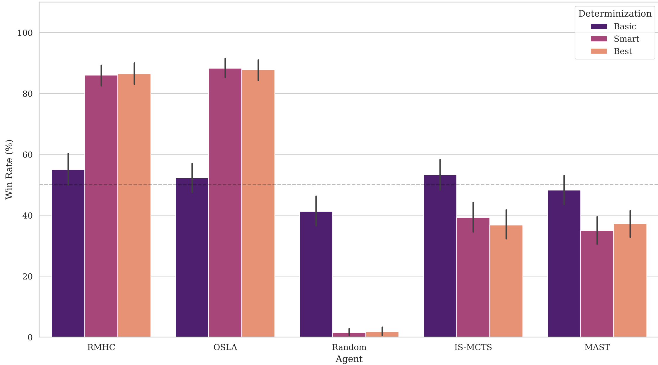
Evolution of Agent Performance across Determinization Modes
