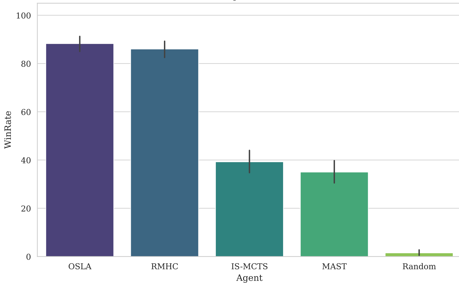
Win Rate Comparison - Smart Mode
