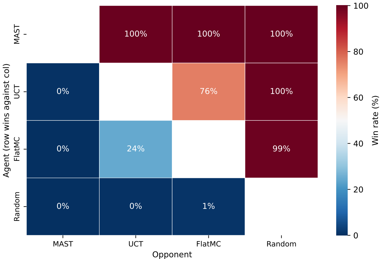
Head-to-head - Tournament 1 (native agents)
