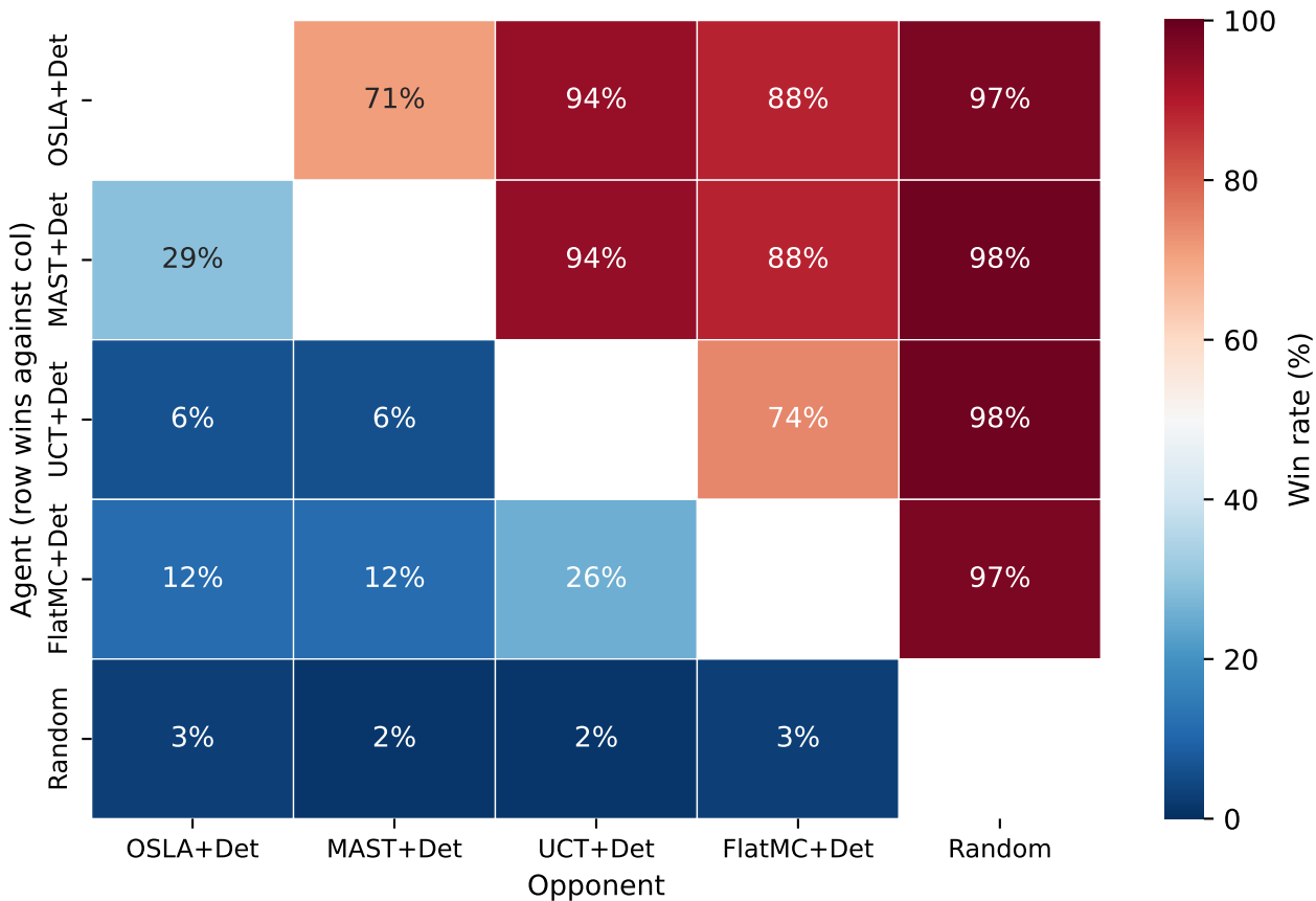
Head-to-head - Tournament 2 (determinized agents)
