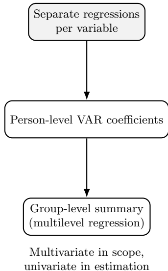
(a) Two-Stage VAR (“mlVAR”) (b) Bayesian Multilevel VAR
