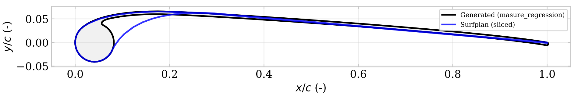
Airfoil 11: t=0.088 , \eta=0.175 , \kappa=0.058 , \delta=4.4^\circ , \lambda=0.100 , \phi=0.650
