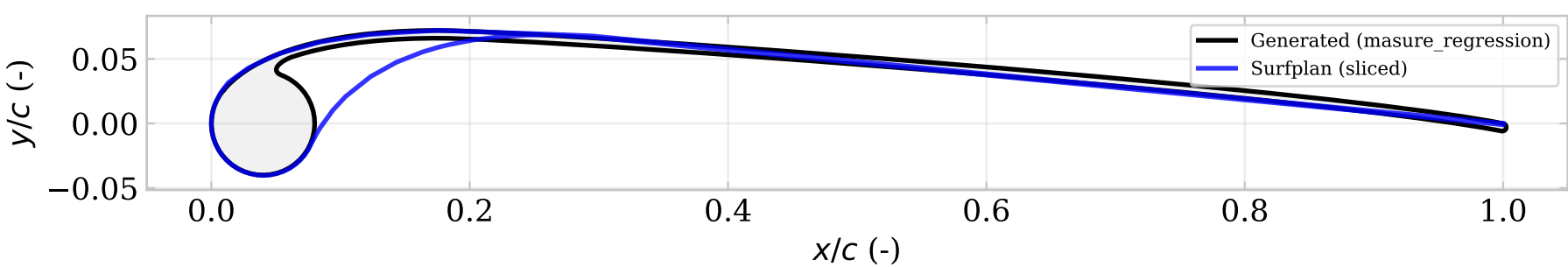
Airfoil 10: t=0.082 , \eta=0.175 , \kappa=0.066 , \delta=5.0^\circ , \lambda=0.100 , \phi=0.650
