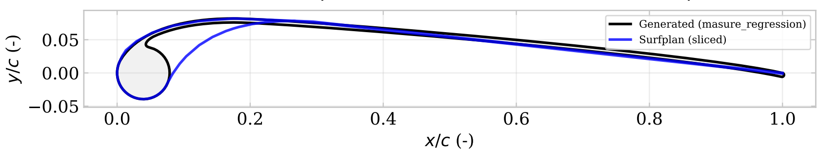
Airfoil 8: t=0.079 , \eta=0.175 , \kappa=0.077 , \delta=5.9^\circ , \lambda=0.100 , \phi=0.650
