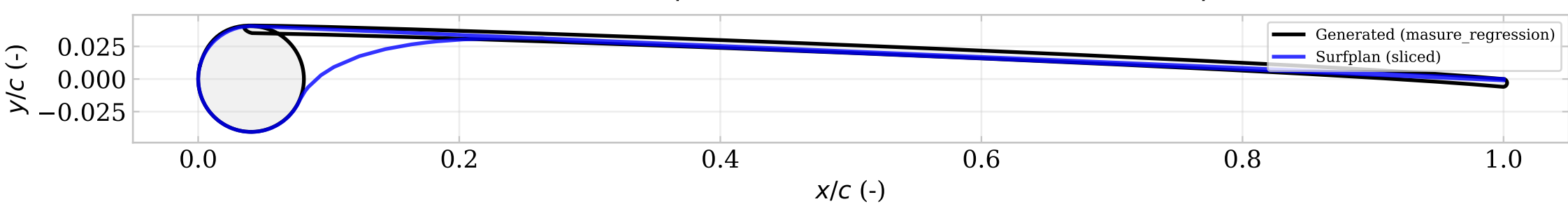
Airfoil 12: t=0.081 , \eta=0.040 , \kappa=0.041 , \delta=2.4^\circ , \lambda=0.100 , \phi=0.650
