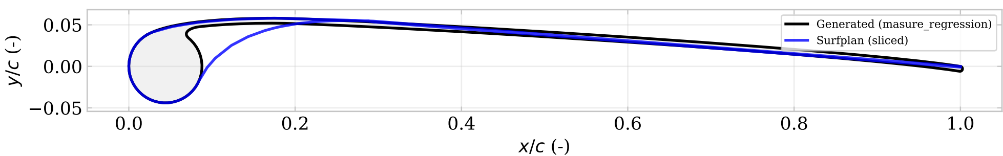
Airfoil 12: t=0.081 , \eta=0.040 , \kappa=0.041 , \delta=2.4^\circ , \lambda=0.100 , \phi=0.650
