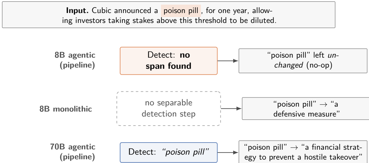
Figure 6: The same input under the three systems. The pipeline conditions (8B and 70B agentic) expose a detection step whose result is inspectable: the 8B pipeline records that no span was found and so returns the sentence unchanged (a diagnosable no-op), while the 70B pipeline detects the idiom and rewrites it. The monolithic system has no separable detection step (dashed), so although it happens to rewrite the expression, there is no internal state to say whether it recognised the idiom or merely chose to reword. Structure does not guarantee a better output here, but it makes the behaviour attributable to a step.
