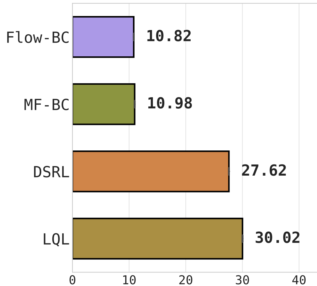
VRAM Consumption (GB ↓)
