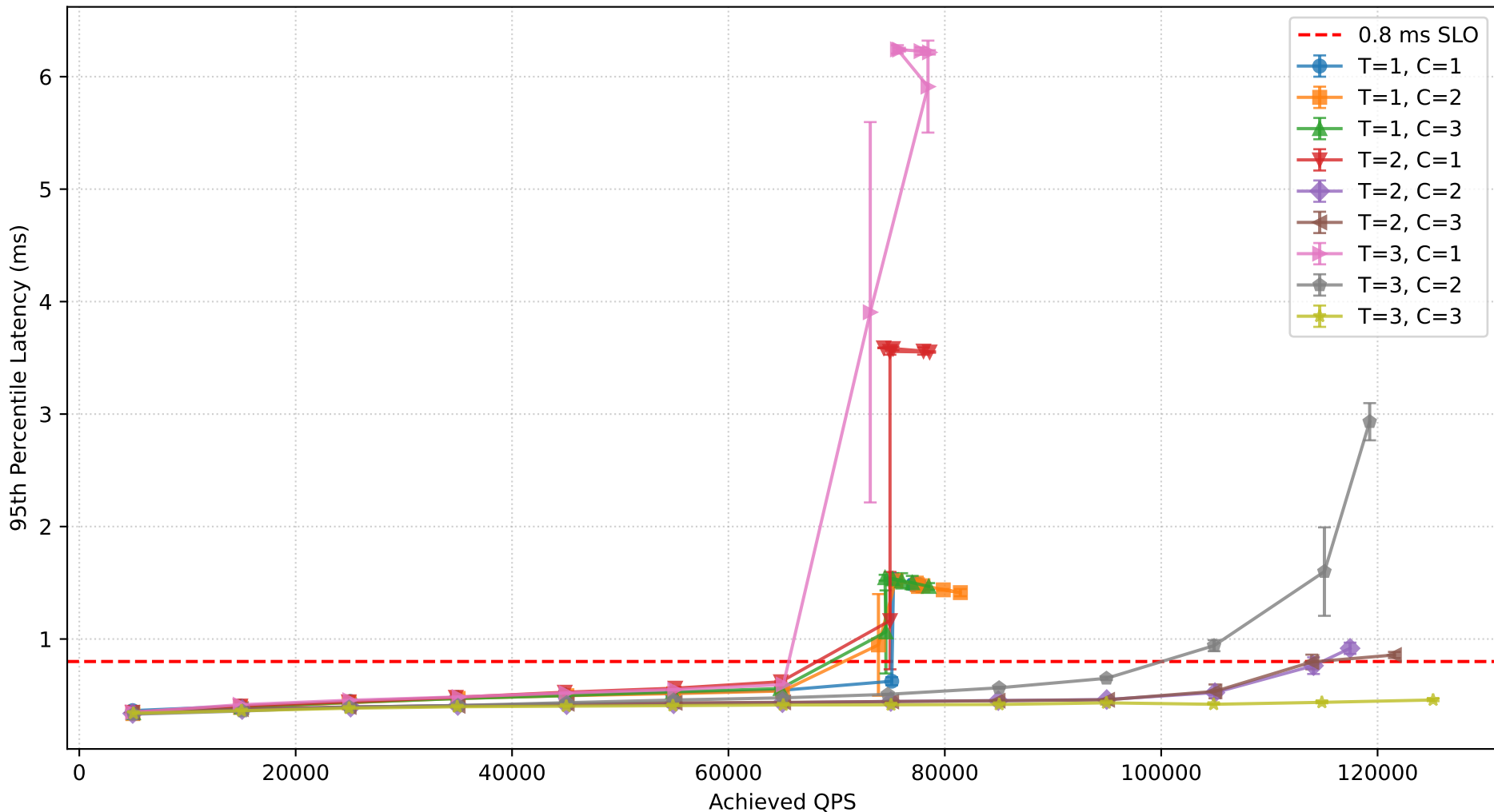
Memcached Performance: 95th Percentile Latency vs. Achieved QPS (Averaged over 3 runs)
