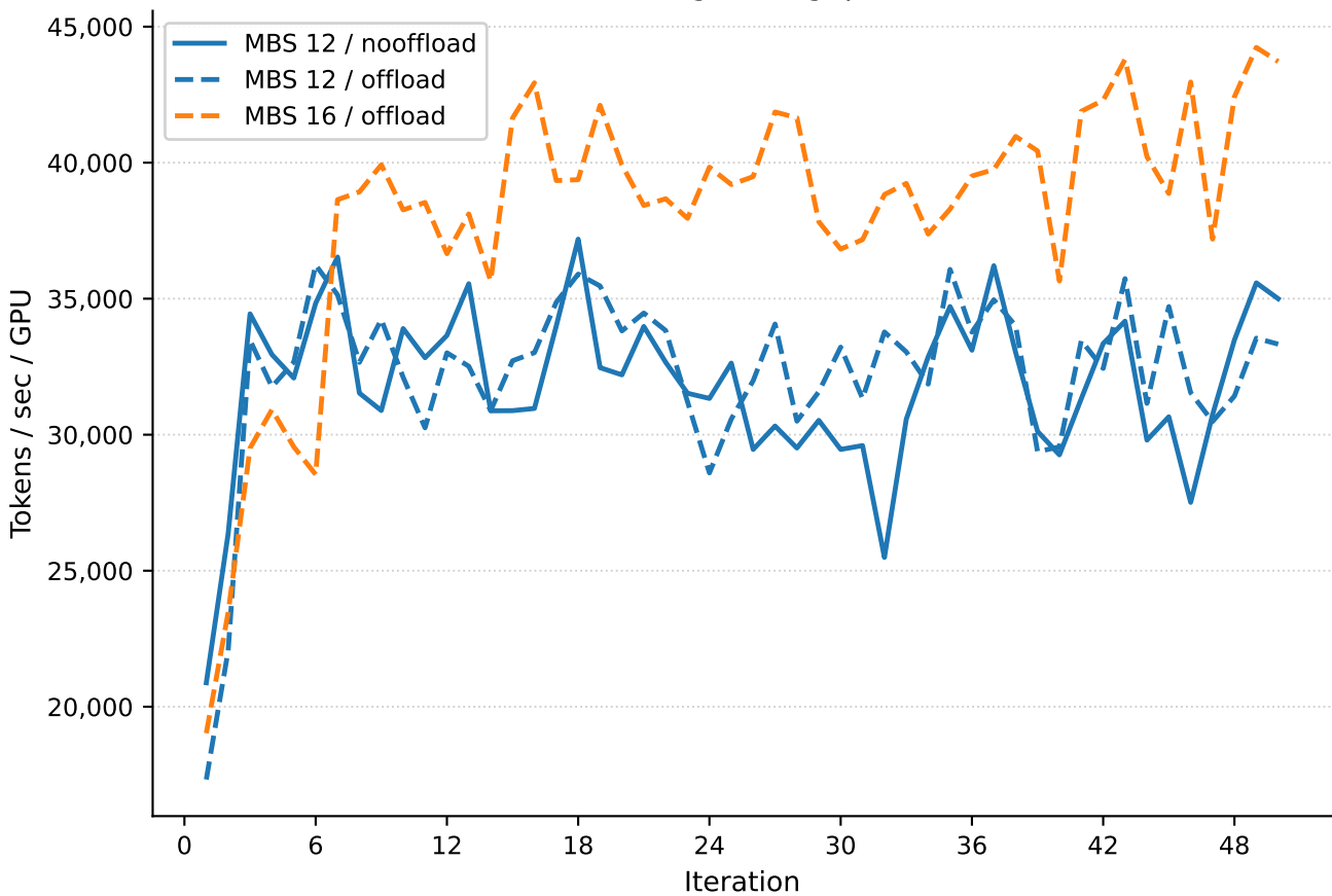
Training Throughput
