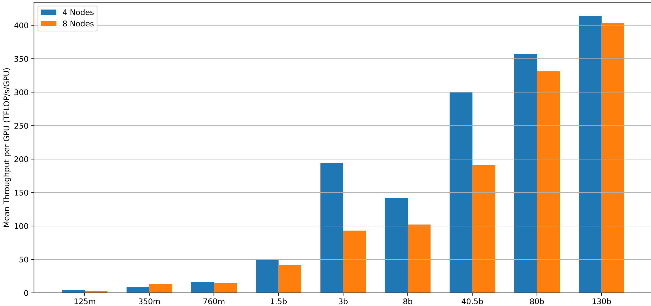
Throughput by Model Size and Number of Nodes (TP=4, PP=4)
