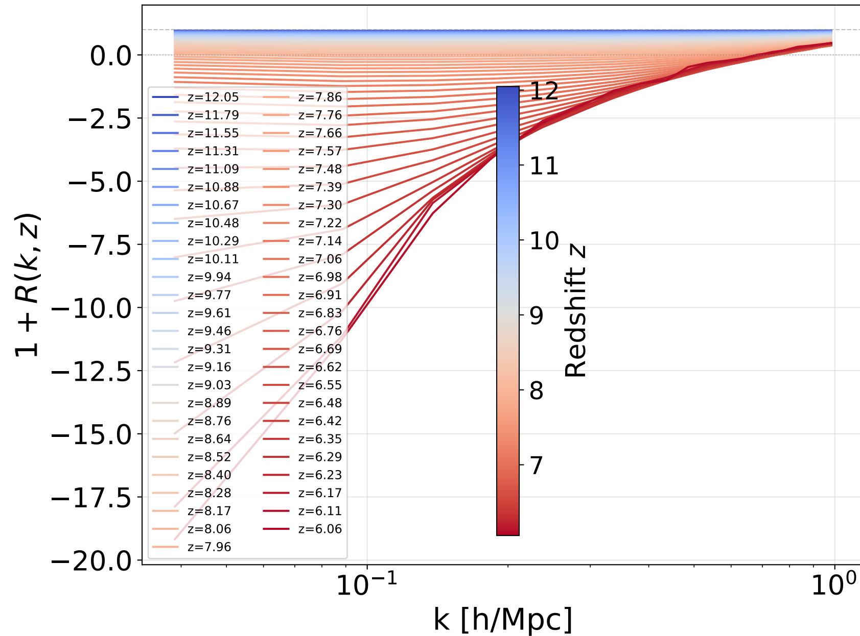
Effective 21cm bias [1 + R(k, z)]
