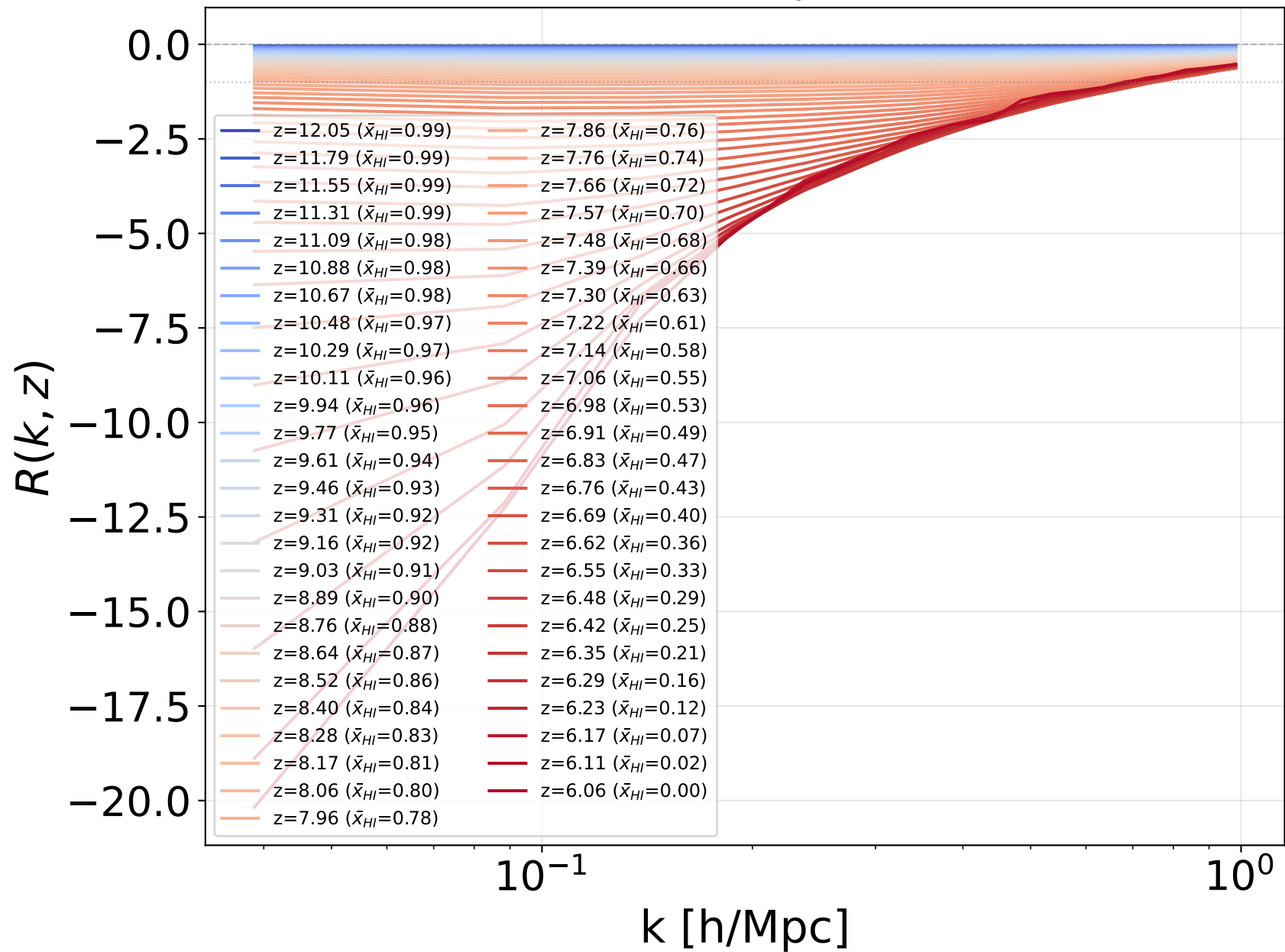
Ionisation-to-density ratio R(k, z)
