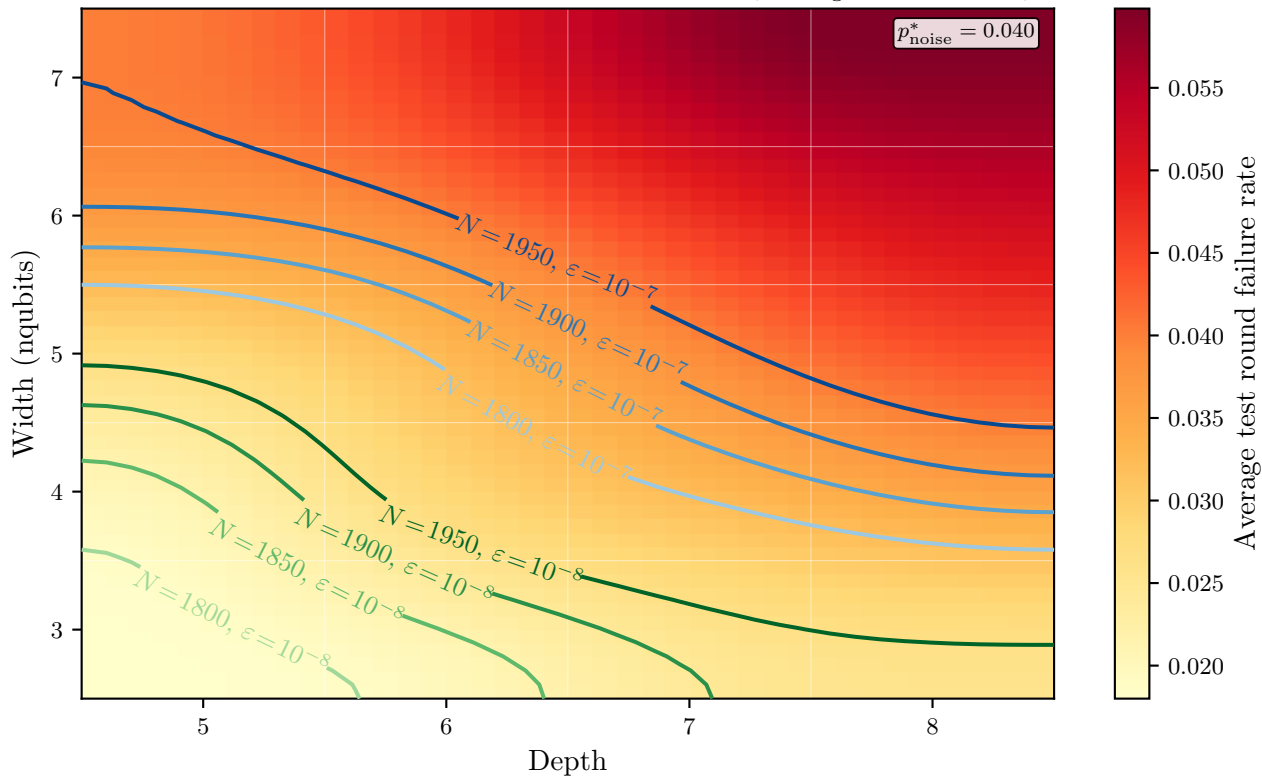
Noise impact on failure rate per circuit dimension ( p_{\text{entagl}} = 0.6 \times 10^{-3} )
