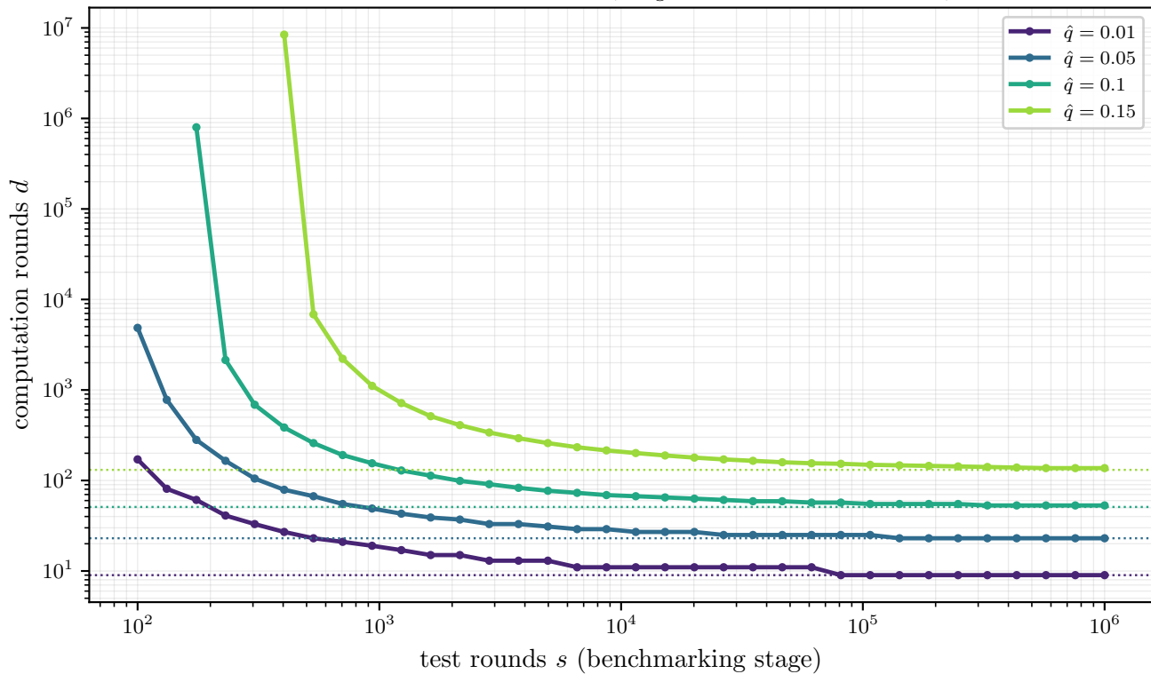
What test rounds buy back ( \epsilon_{\text{target}} = 10^{-6} , k = 2 , c = 0.0 )
