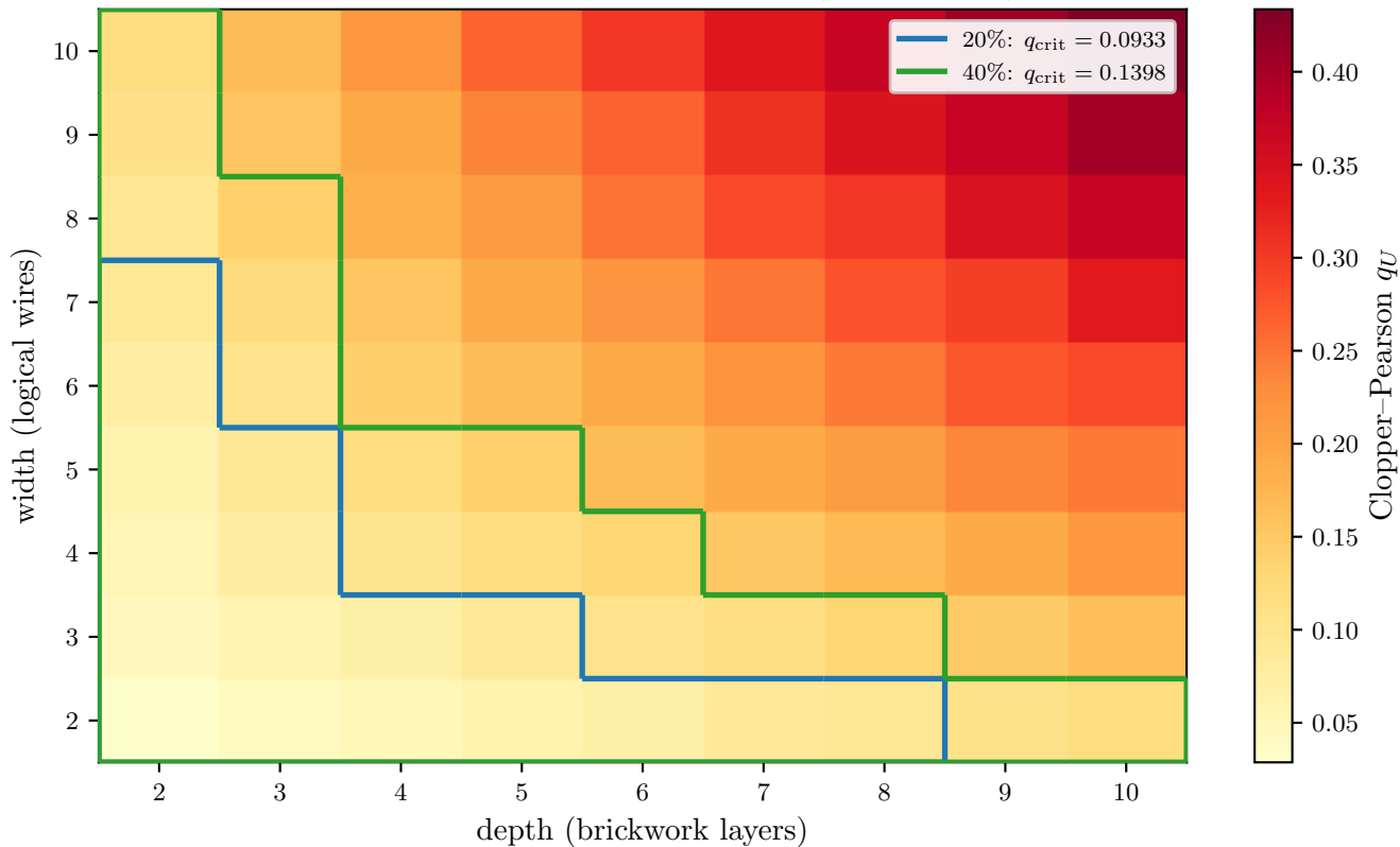
Verifiable quantum volume: certification frontiers ( p = 1.0e - 03 ), s=10000
