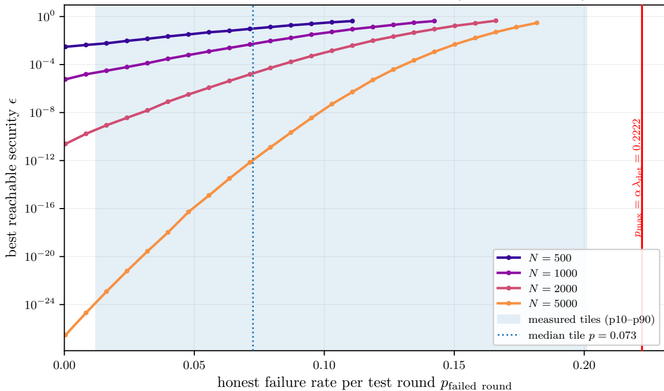
Cost-driven: security reachable at fixed budget ( c = 0.1 , \lambda_{\text{det}} = 0.5 )
