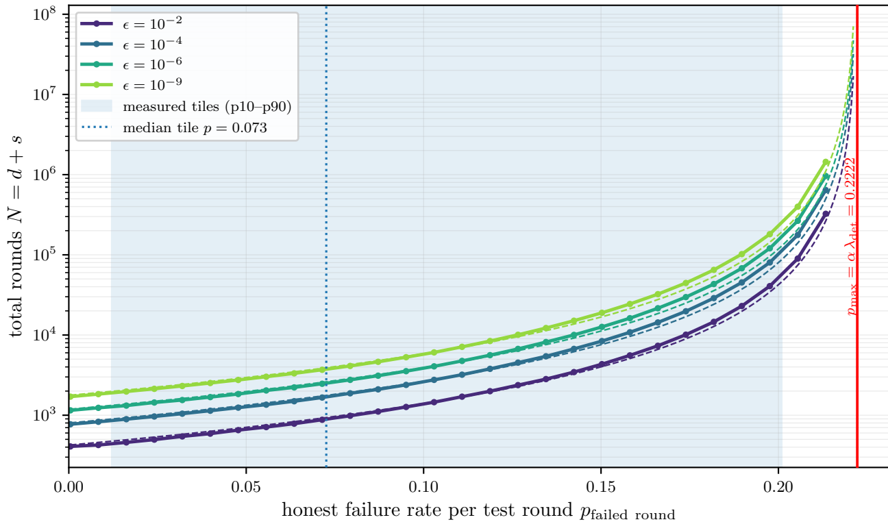
Performance-driven: rounds needed at fixed security ( c = 0.1 , \lambda_{\text{det}} = 0.5 )
