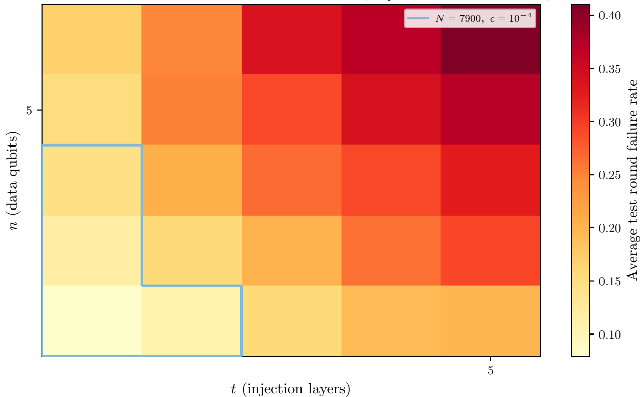
Noise impact on failure rate per circuit dimension ( p_{\text{depol}} = 10^{-2} , N_{\text{shots}} = 100 )
