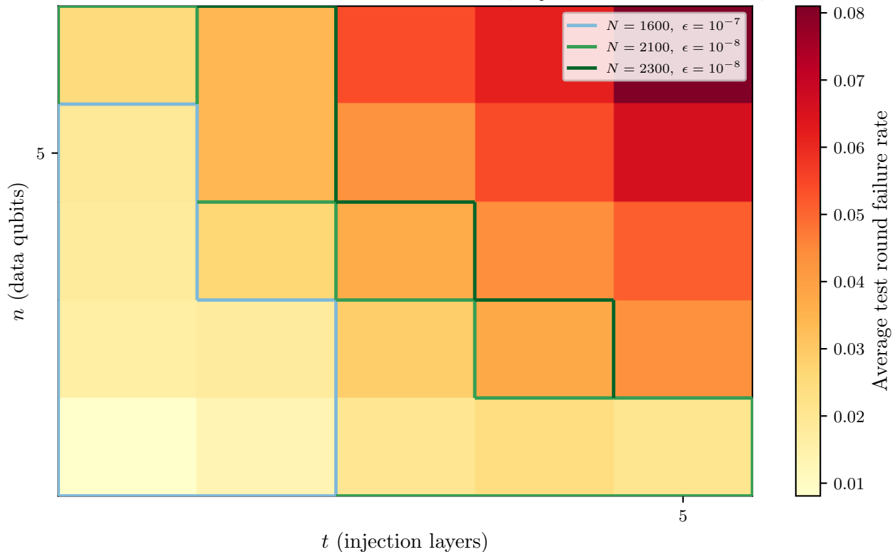
Noise impact on failure rate per circuit dimension ( p_{\text{depol}} = 10^{-3} , N_{\text{shots}} = 100 )
