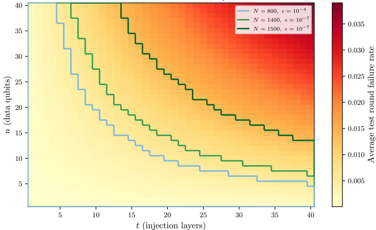
Noise impact on failure rate per circuit dimension ( p_{\text{depol}} = 10^{-5} , N_{\text{shots}} = 10000 )
