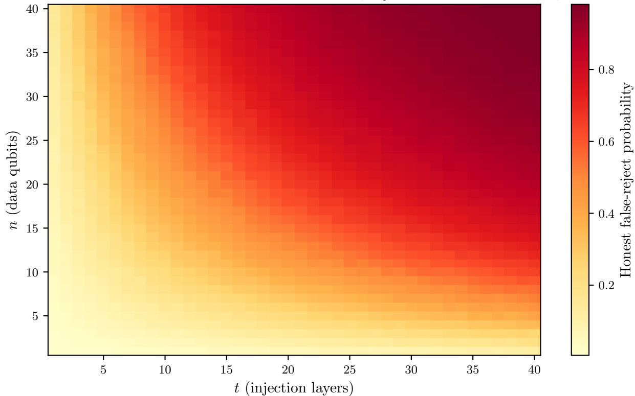
Noise impact on failure rate per circuit dimension ( p_{\text{depol}} = 10^{-5} , N_{\text{shots}} = 10000 )
