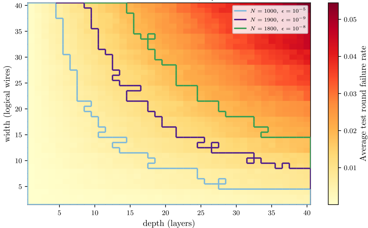
Noise impact on failure rate per circuit dimension ( p_{\text{depol}} = 1.5 \times 10^{-5} , N_{\text{shots}} = 1000 )
