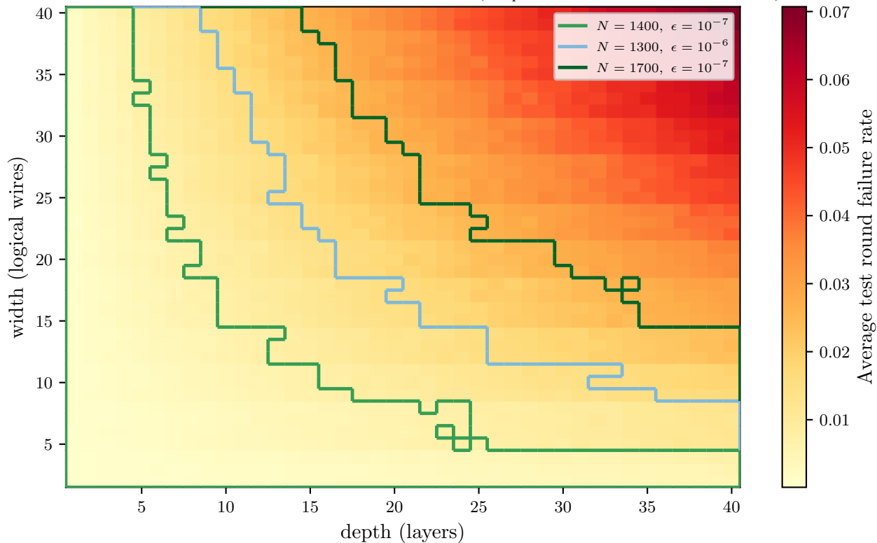
Noise impact on failure rate per circuit dimension ( p_{\text{depol}} = 2 \times 10^{-5} , N_{\text{shots}} = 1000 )
