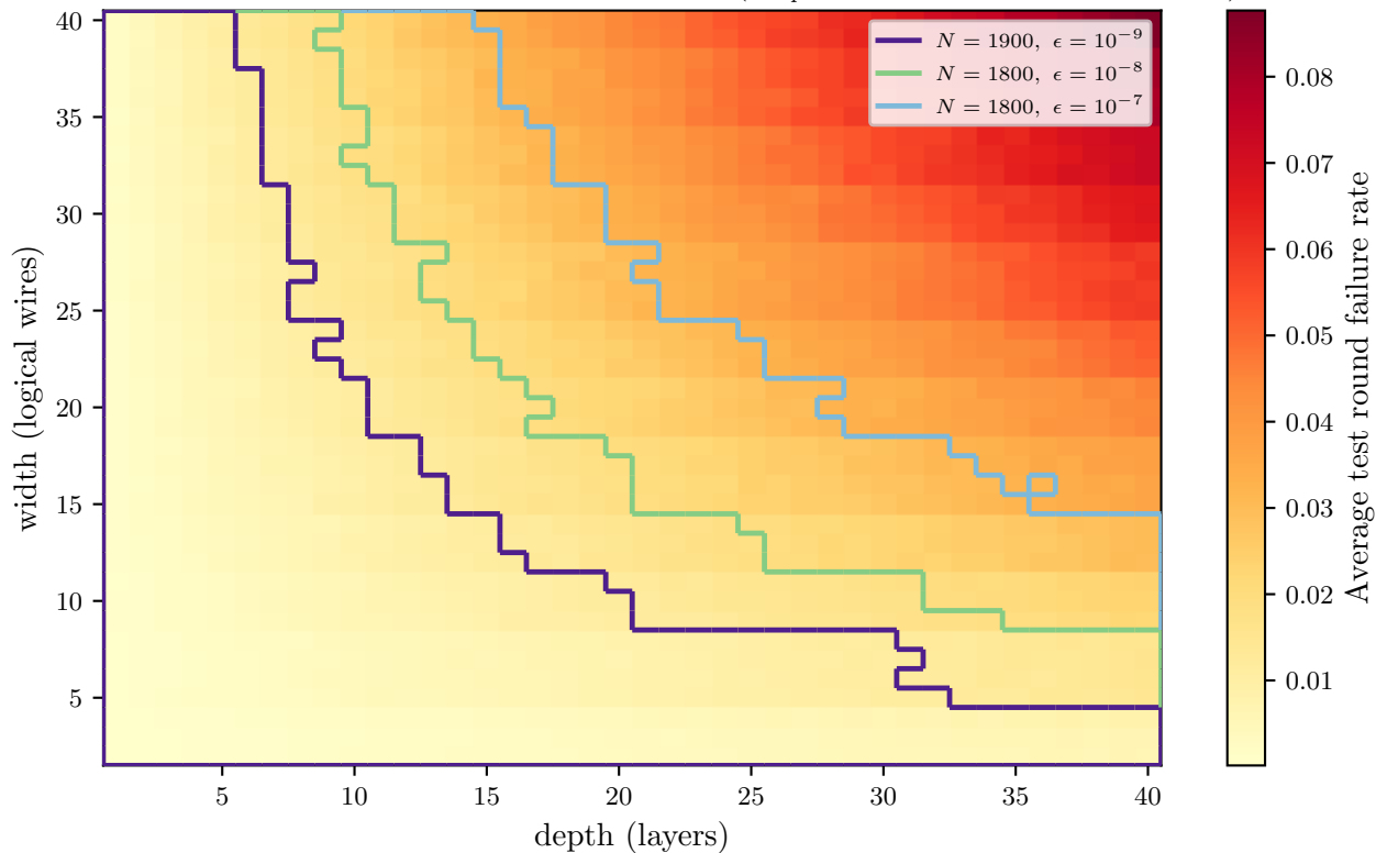
Noise impact on failure rate per circuit dimension ( p_{\text{depol}} = 2.5 \times 10^{-5} , N_{\text{shots}} = 1000 )
