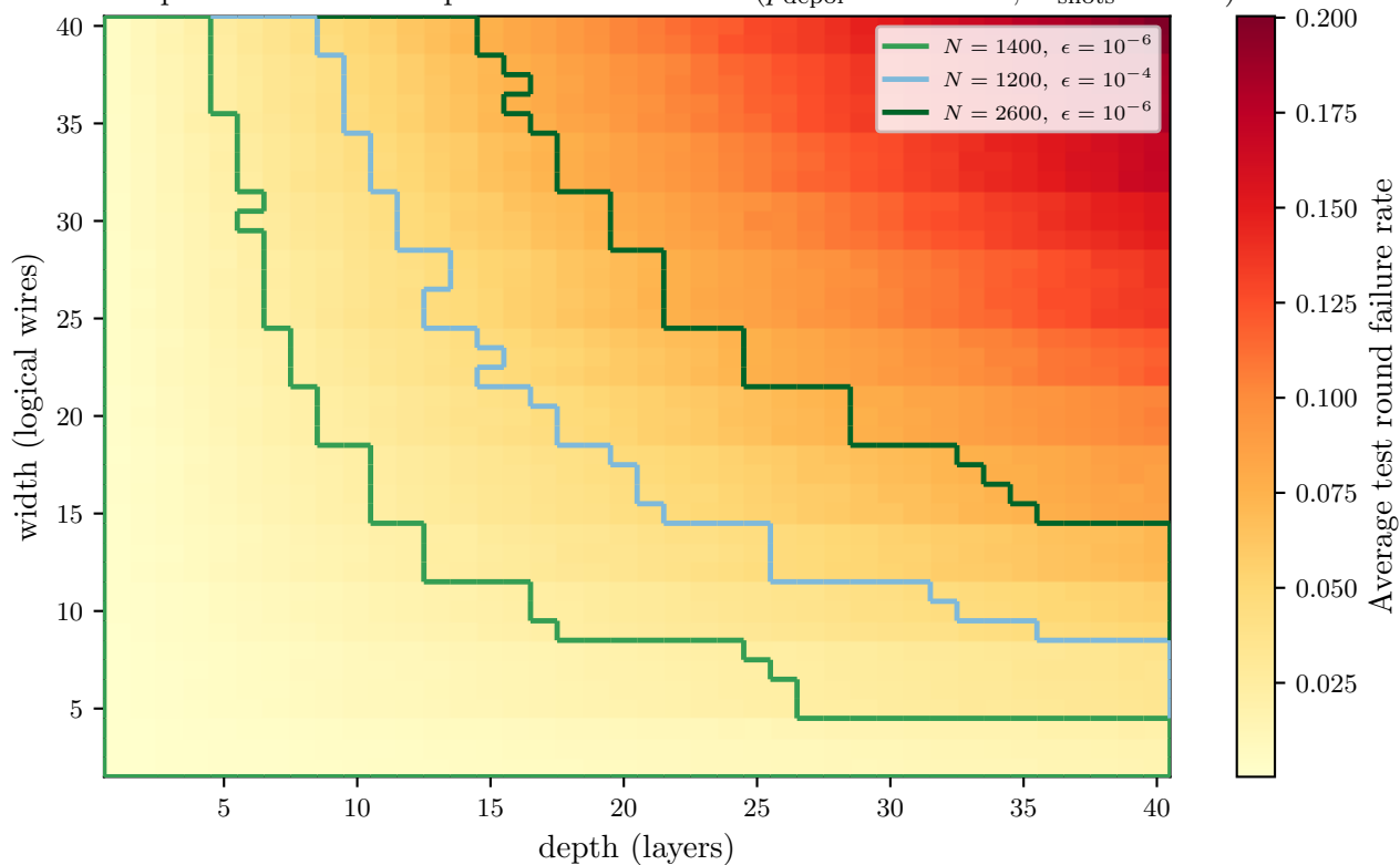
Noise impact on failure rate per circuit dimension ( p_{\text{depol}} = 6 \times 10^{-5} , N_{\text{shots}} = 1000 )
