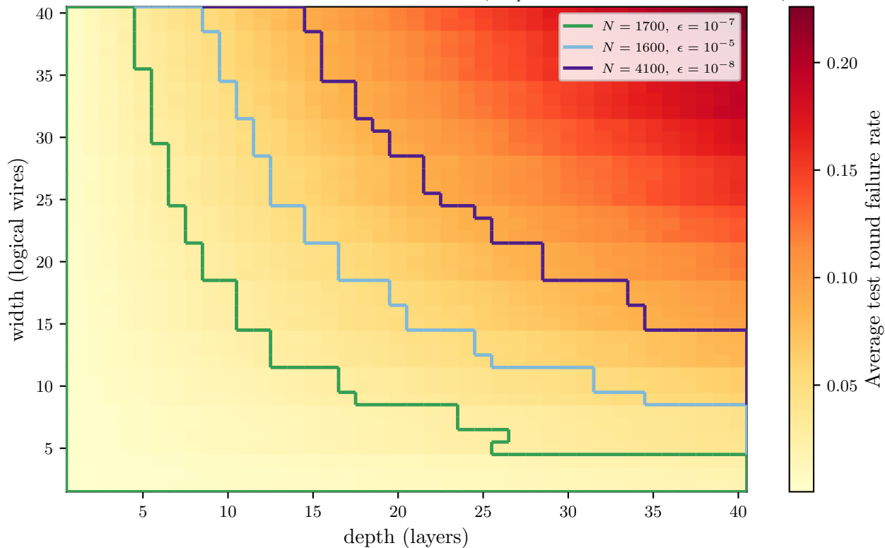
Noise impact on failure rate per circuit dimension ( p_{\text{depol}} = 7 \times 10^{-5} , N_{\text{shots}} = 1000 )
