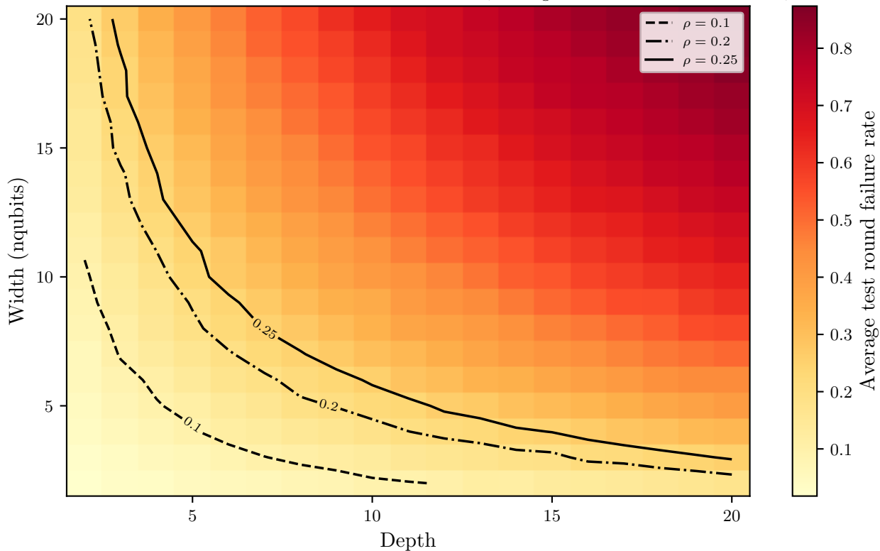
Noise impact on failure rate per circuit dimension ( p_{\text{entangle}} = 10^{-3} , N_{\text{rounds}} = 10000 )
