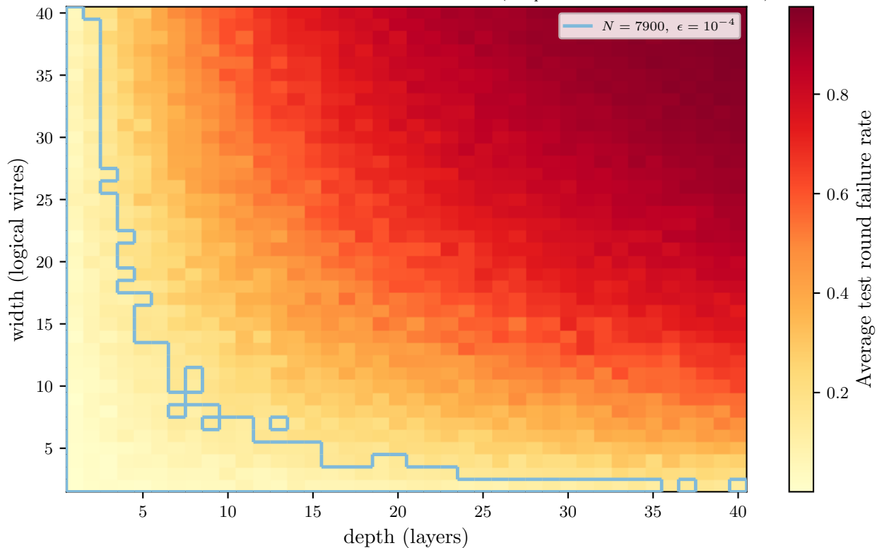
Noise impact on failure rate per circuit dimension ( p_{\text{depol}} = 10^{-3} , N_{\text{shots}} = 1000 )
