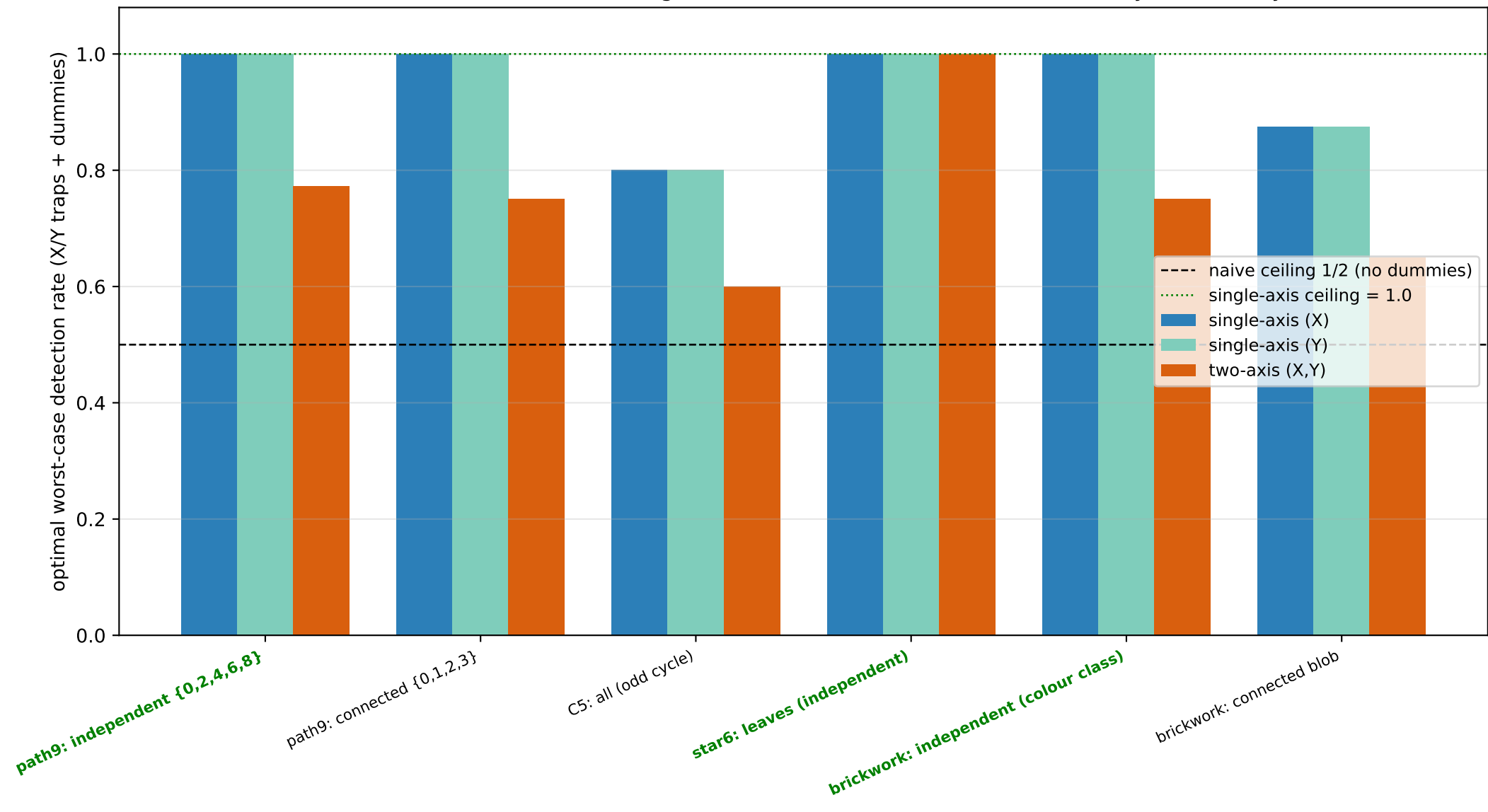
Harmful-noise detection (blind MBQC): single-axis \rightarrow 1.0 ; two-axis lifted above 1/2 by the dummy mechanism
