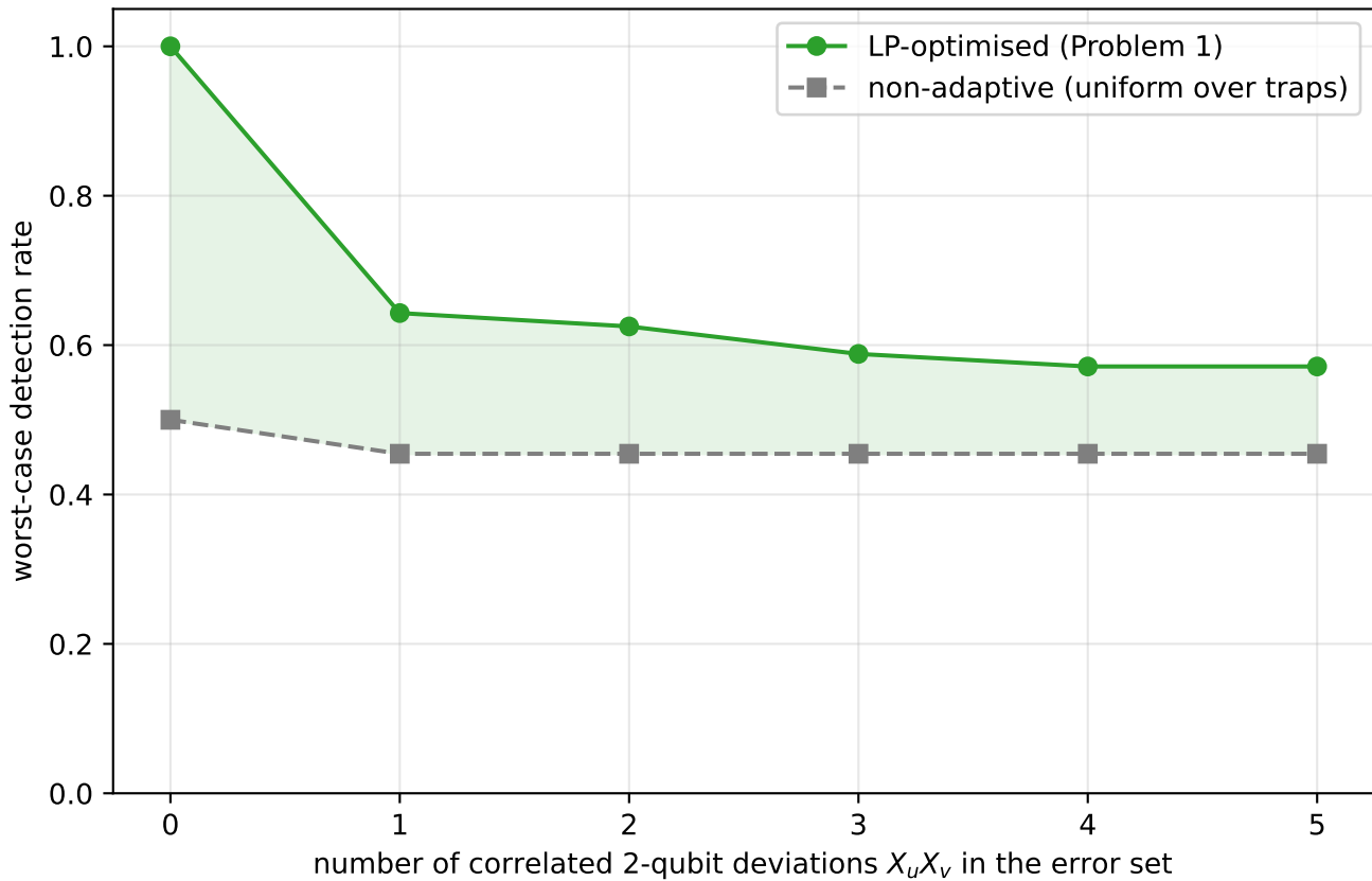
General deviations: the LP adapts to the error structure (mixed single-qubit X/Y + correlated 2-qubit; physical X/Y traps + dummies)
