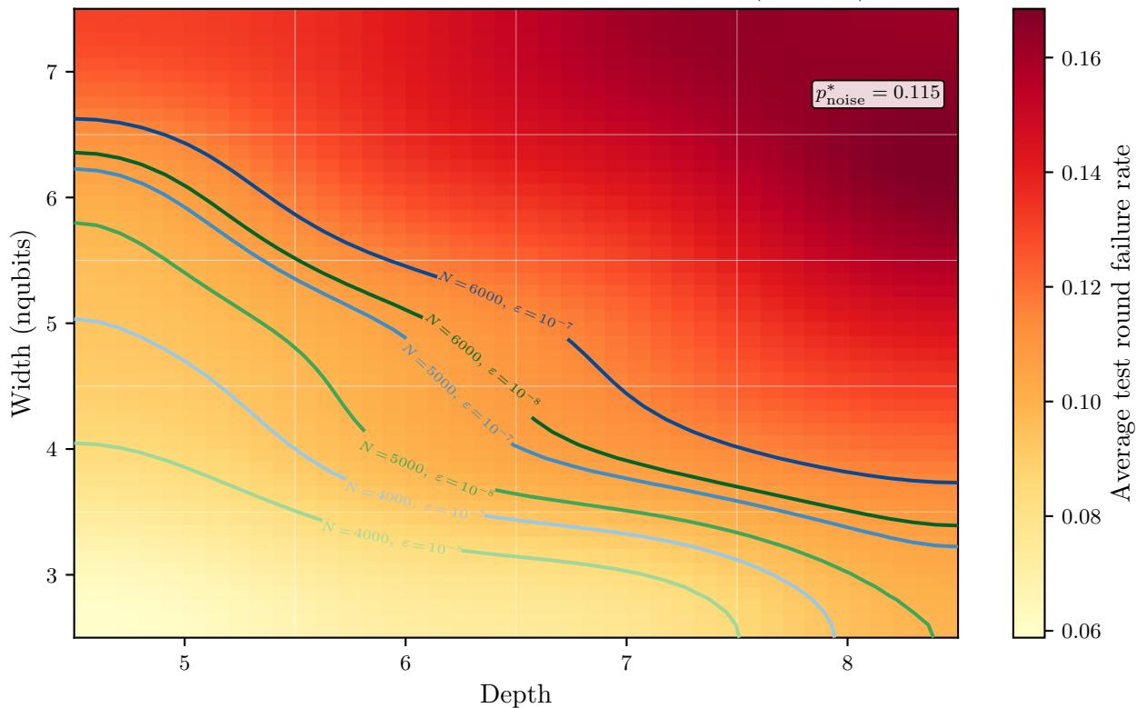
Noise impact on failure rate per circuit dimension ( p=2e-03 )
