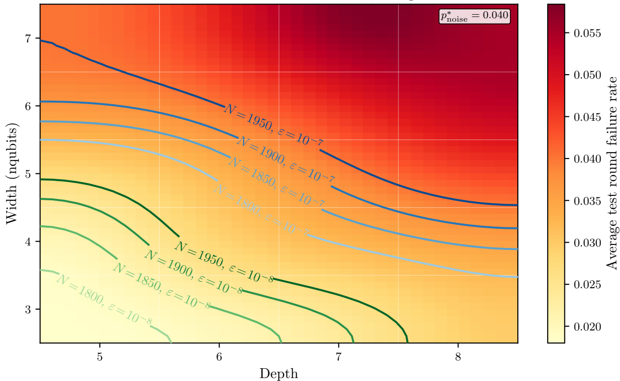
Noise impact on failure rate per circuit dimension ( p_{\text{entangl}} = 0.6 \times 10^{-3} )
