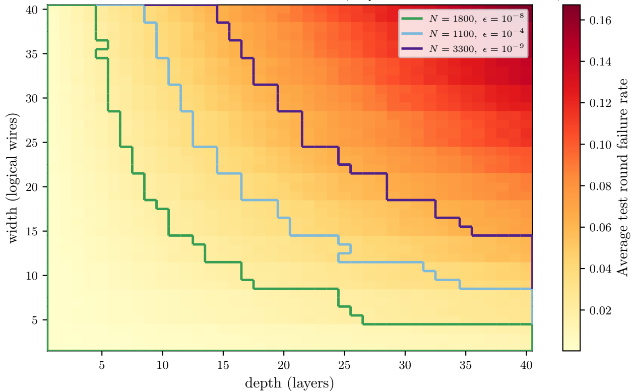
Noise impact on failure rate per circuit dimension ( p_{\text{depol}} = 5 \times 10^{-5} , N_{\text{shots}} = 1000 )
