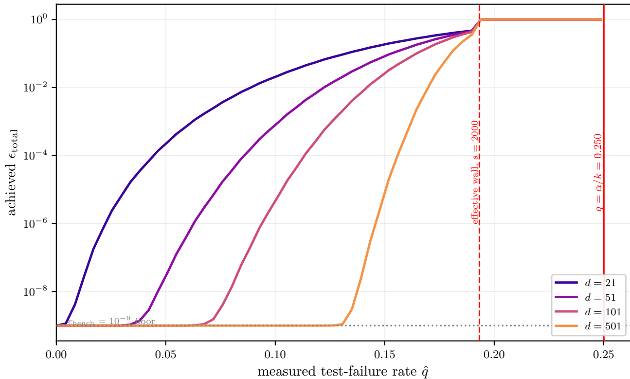
Cost-driven: correctness at fixed budget ( s = 2000 , k = 2 , c = 0.0 )
