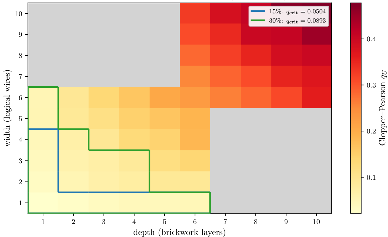
Verifiable quantum volume: certification frontiers ( p = 1.0e - 03 ), s=2000
