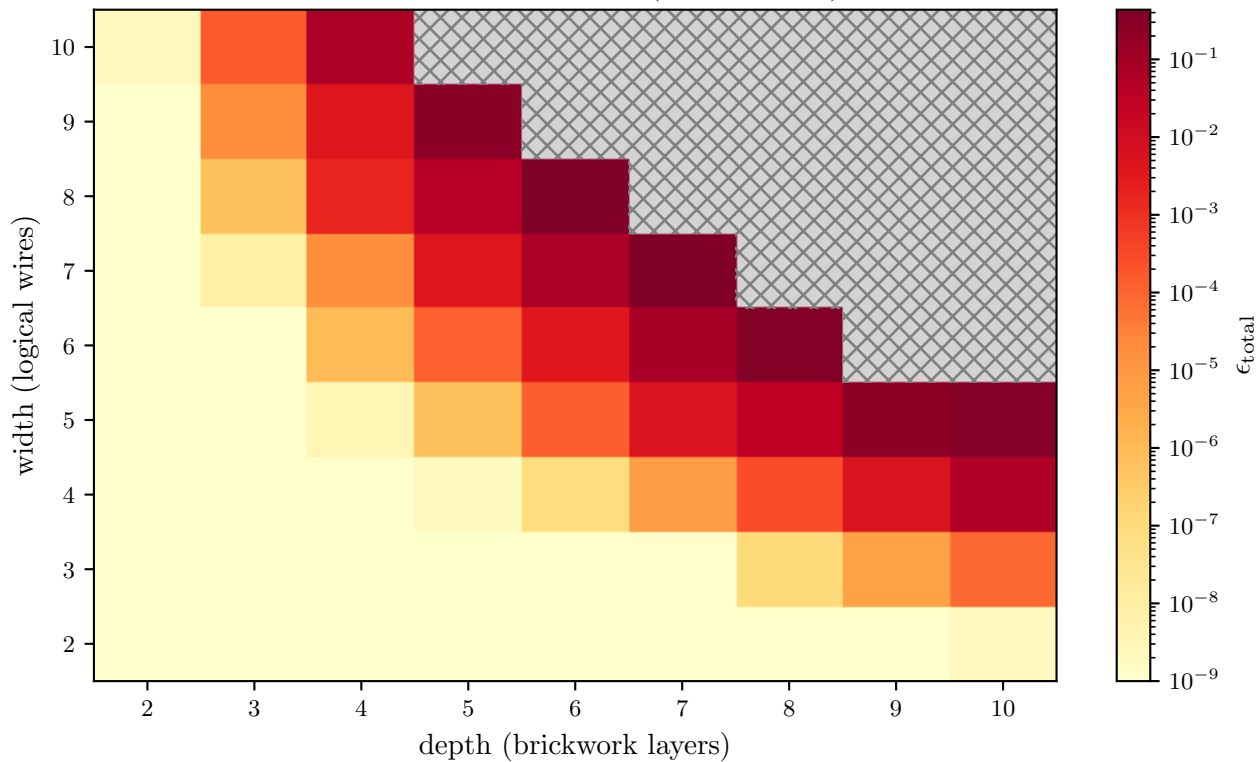
Achieved \epsilon_{\text{total}} at d = 101 ( p = 1.0e - 03 )
