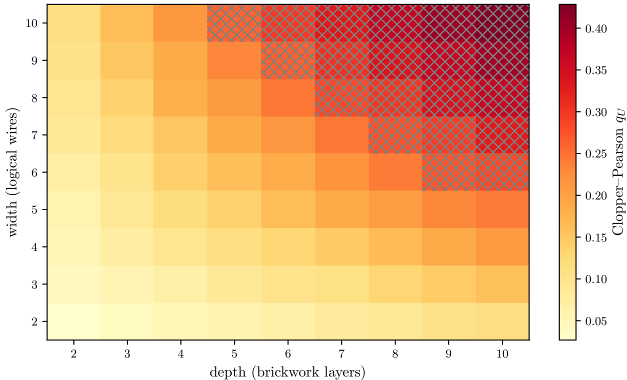
Noise bound q_U per circuit dimension ( p = 1.0e - 03 ), s=10000
