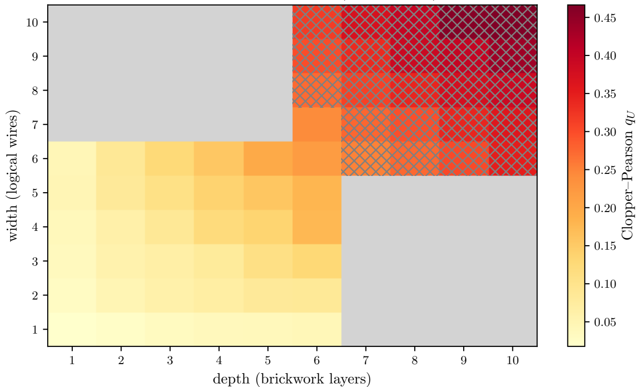
Noise bound q_U per circuit dimension ( p = 1.0e - 03 ), s=2000
