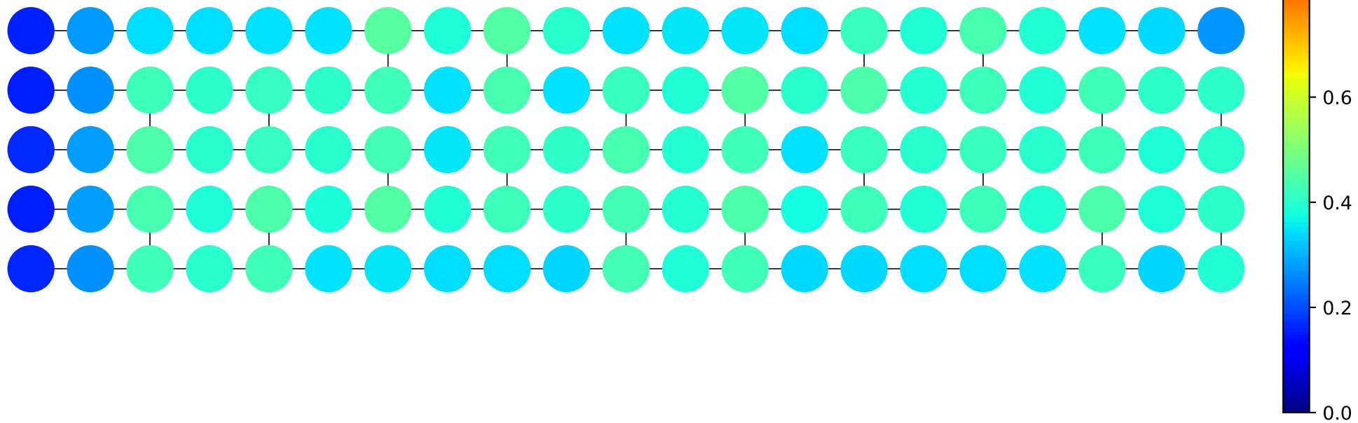
FK12 trap failure rate (n=5, d=21, 100 circuits × 100 rounds, depolarising, p_{\text{ent}}=3\text{e-}01 )
