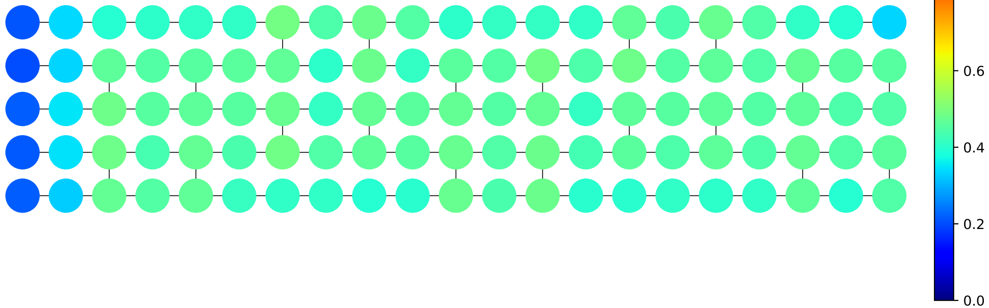
FK12 trap failure rate (n=5, d=21, 100 circuits \times 100 rounds, depolarising, p_{\text{ent}}=4\text{e-}01 )
