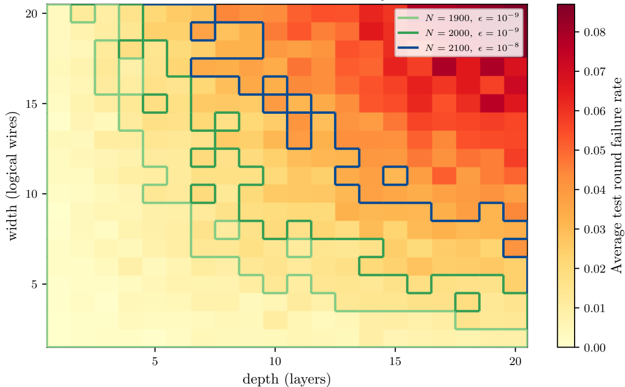
Noise impact on failure rate per circuit dimension ( p_{\text{depol}} = 10^{-4} , N_{\text{shots}} = 100 )
