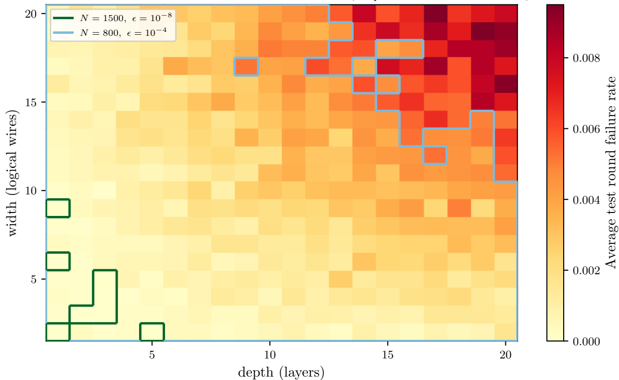
Noise impact on failure rate per circuit dimension ( p_{\text{depol}} = 10^{-5} , N_{\text{shots}} = 100 )
