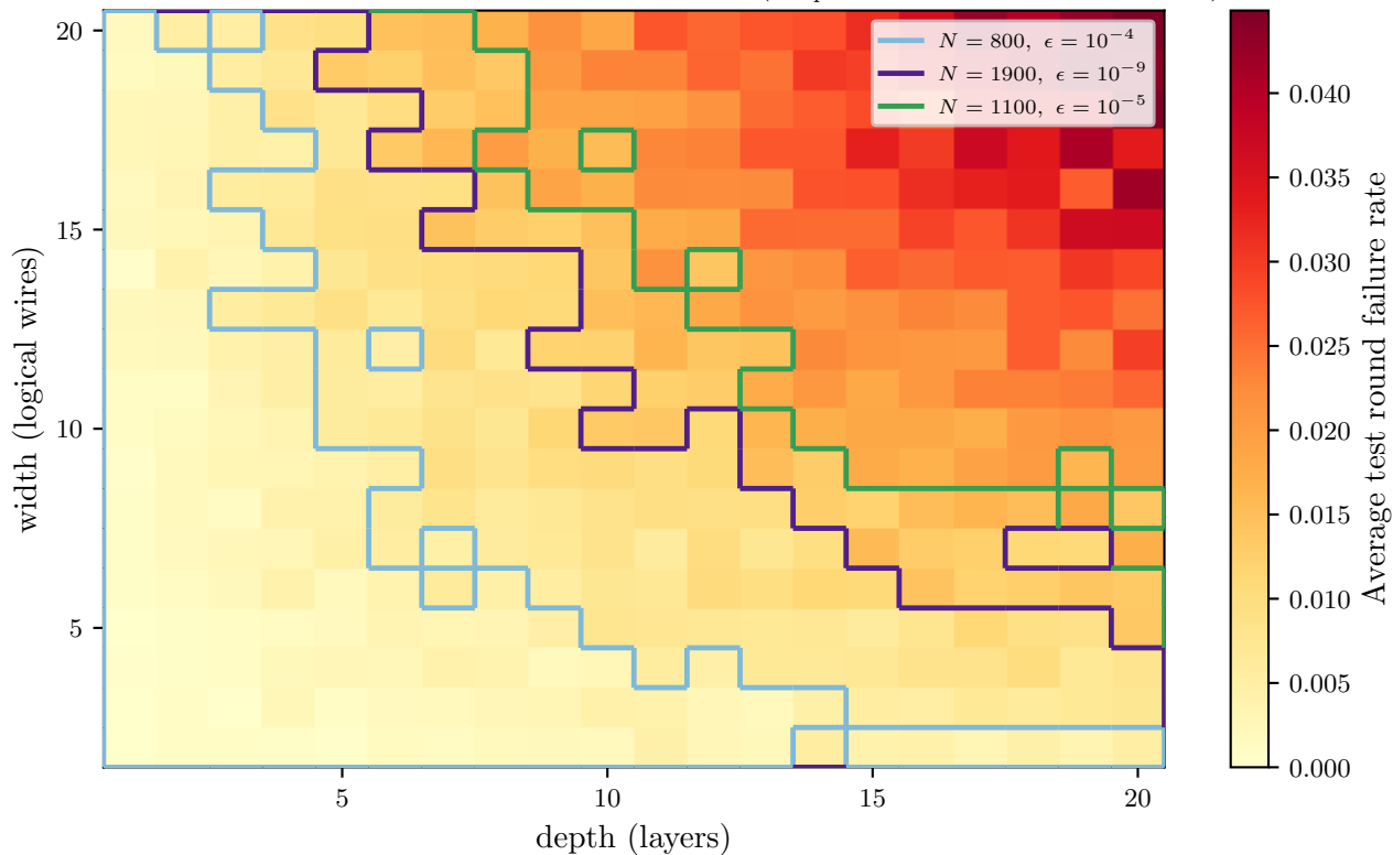
Noise impact on failure rate per circuit dimension ( p_{\text{depol}} = 5 \times 10^{-5} , N_{\text{shots}} = 100 )
