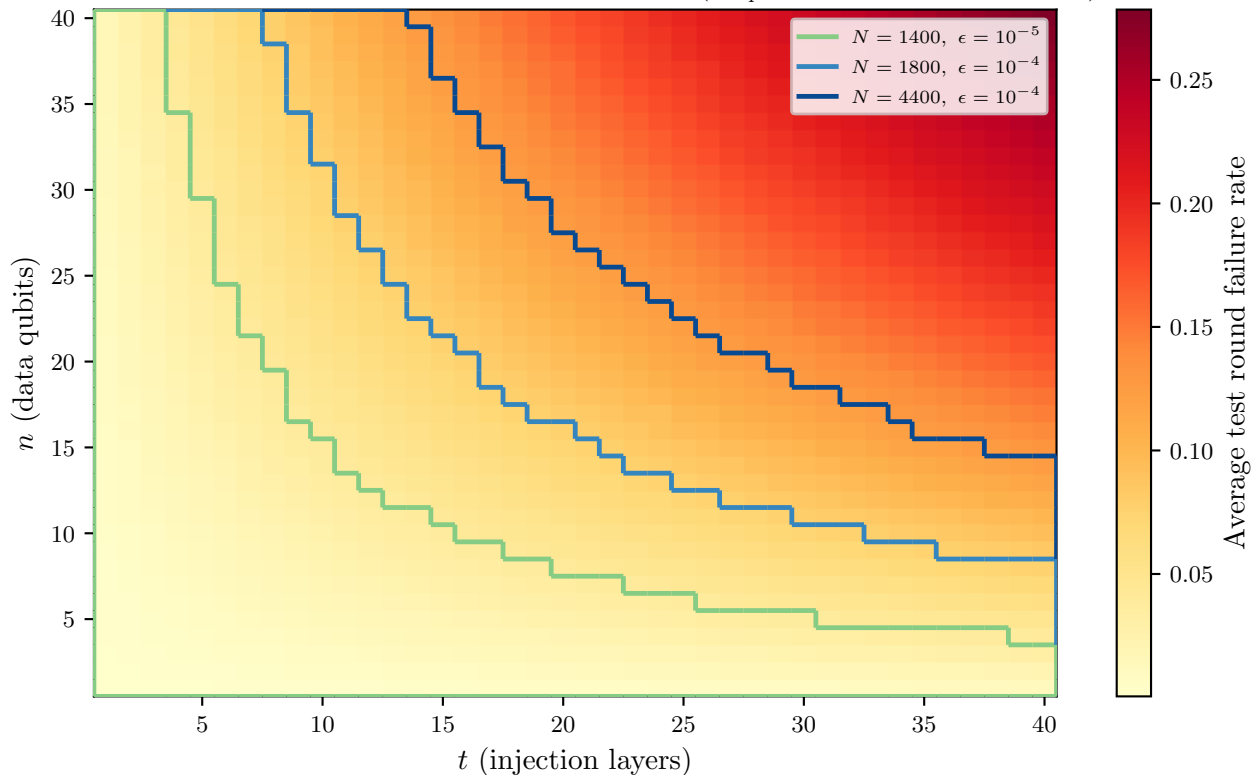
Noise impact on failure rate per circuit dimension ( p_{\text{depol}} = 10^{-4} , N_{\text{shots}} = 10000 )
