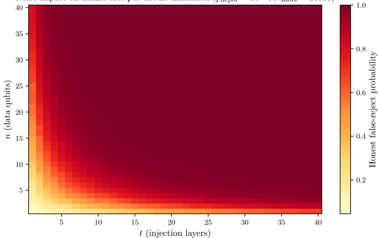
Noise impact on failure rate per circuit dimension ( p_{\text{depol}} = 10^{-4} , N_{\text{shots}} = 10000 )
