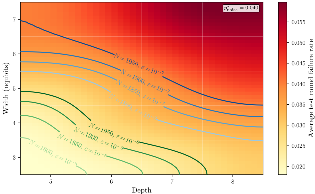
Noise impact on failure rate per circuit dimension ( p_{\text{entangle}} = 0.6 \times 10^{-3} )
