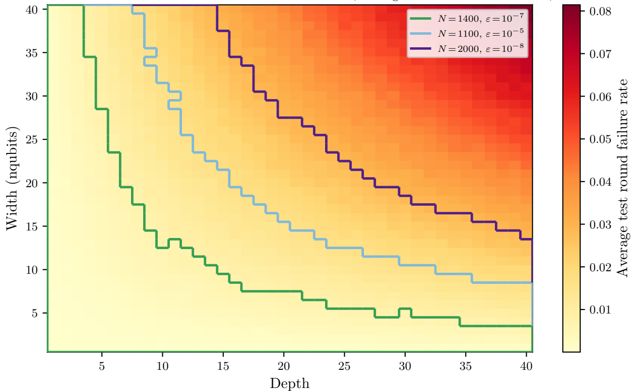
Noise impact on failure rate per circuit dimension ( p_{\text{entangle}} = 10^{-5} , N_{\text{shots}} = 1000 )
